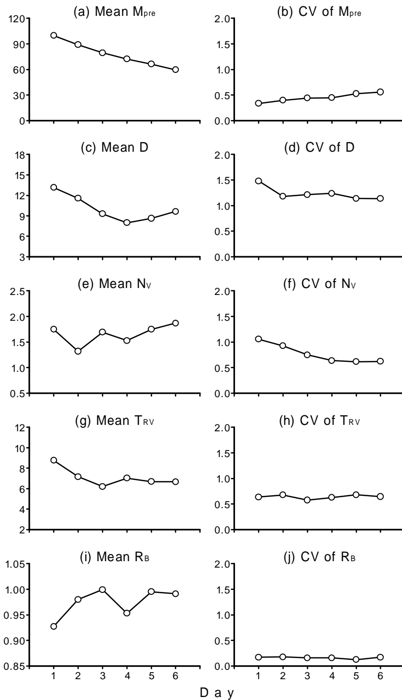
Figure 2. Changes in the mean and coefficient of variation (CV, fraction) of pre-grazing herbage mass ( M_{pre} ), rate of defoliation ( D ), number of visits ( N_v ), residence time per visit ( T_{RV} ) and rate of biting ( R_B ) with the progress of grazing (Days 1 to 6). The unit of the mean is g DM ( 2500 \text{ cm}^2 ) -1 for M_{pre} , g DM ( 2500 \text{ cm}^2 ) -1 d -1 for D , visits ( 2500 \text{ cm}^2 ) -1 d -1 for N_v , s visit -1 for T_{RV} and bites s -1 for R_B .
