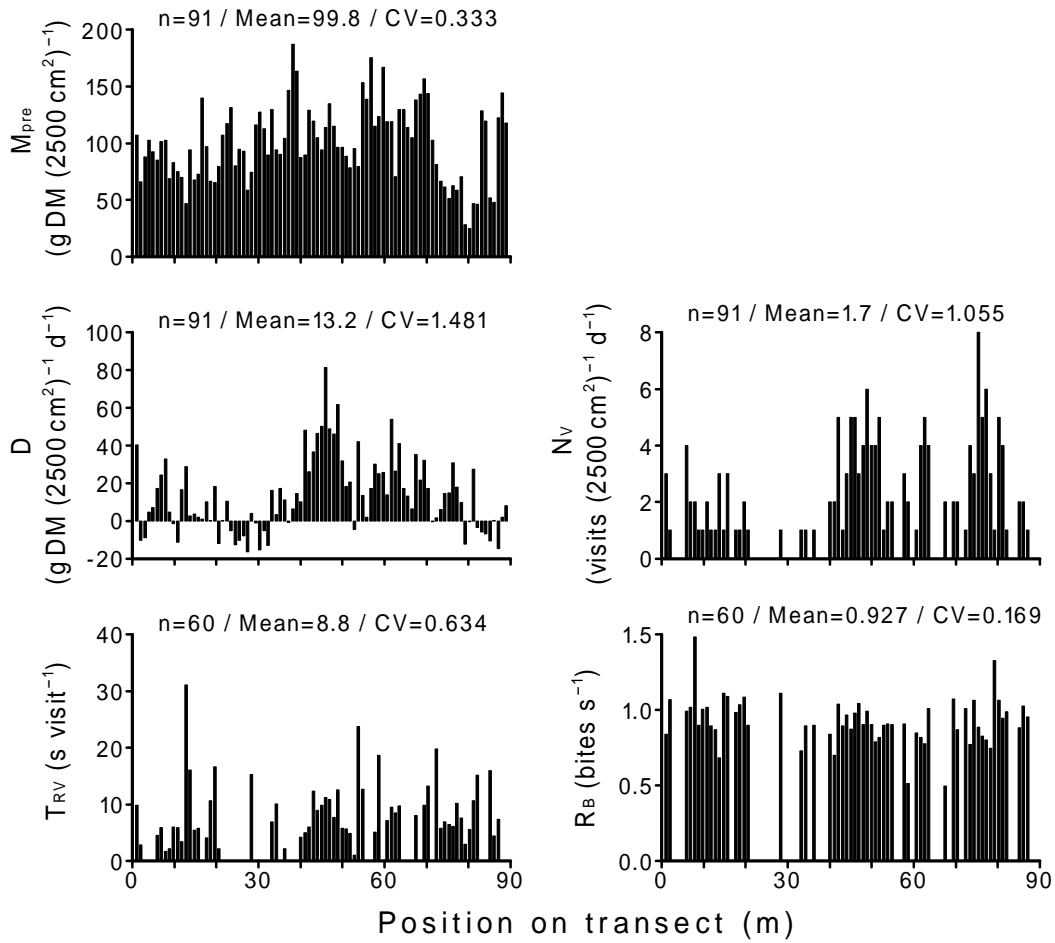
Figure 1. Spatial distribution of pre-grazing herbage mass ( M_{pre} ), rate of defoliation ( D ), number of visits ( N_v ), residence time per visit ( T_{RV} ) and rate of biting ( R_B ) along the transect on Day 1. The statistical parameters are the number of samples ( n ), mean and coefficient of variation (CV, fraction).
